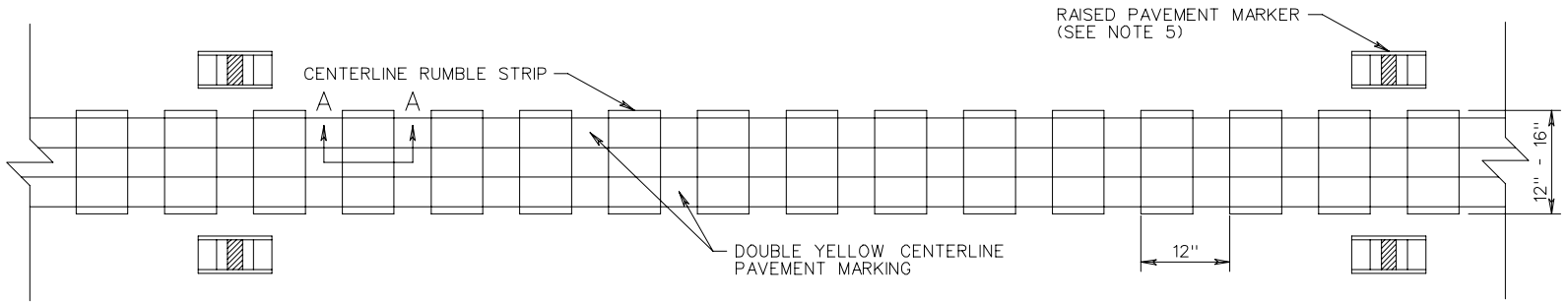
PLAN VIEW
