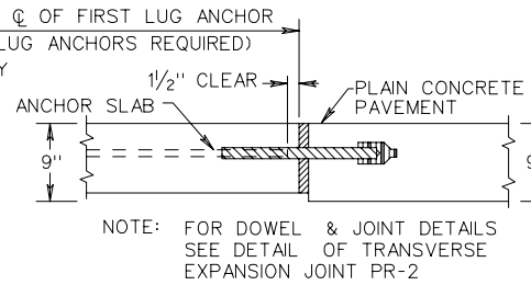
SECTION B-B ANCHOR SLAB TYPE I (FOR USE ADJACENT TO PLAIN CONCRETE PAVEMENT)
