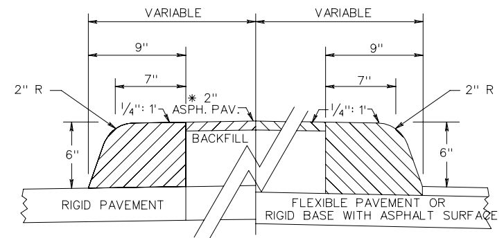
ASPHALT MEDIAN
