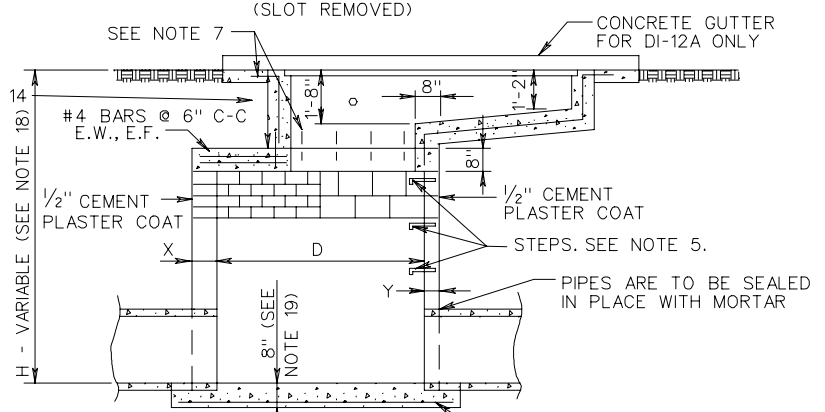
HALF SECTION HALF SECTION BRICK CONCRETE BLOCK
