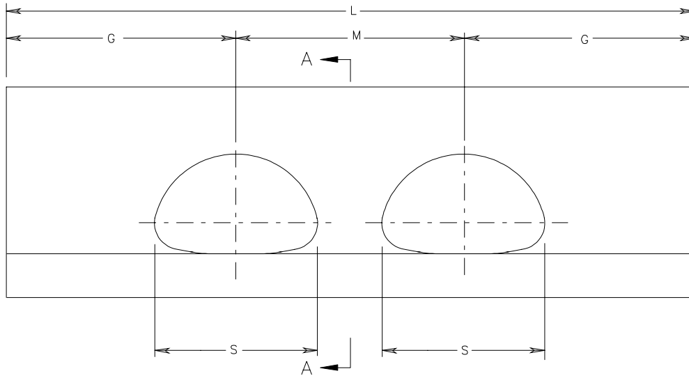
FRONT ELEVATION
