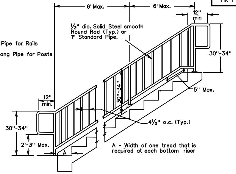
HANDRAIL INSTALLATION
