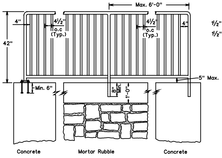
HANDRAIL (GUARD) INSTALLATION ON WALLS
