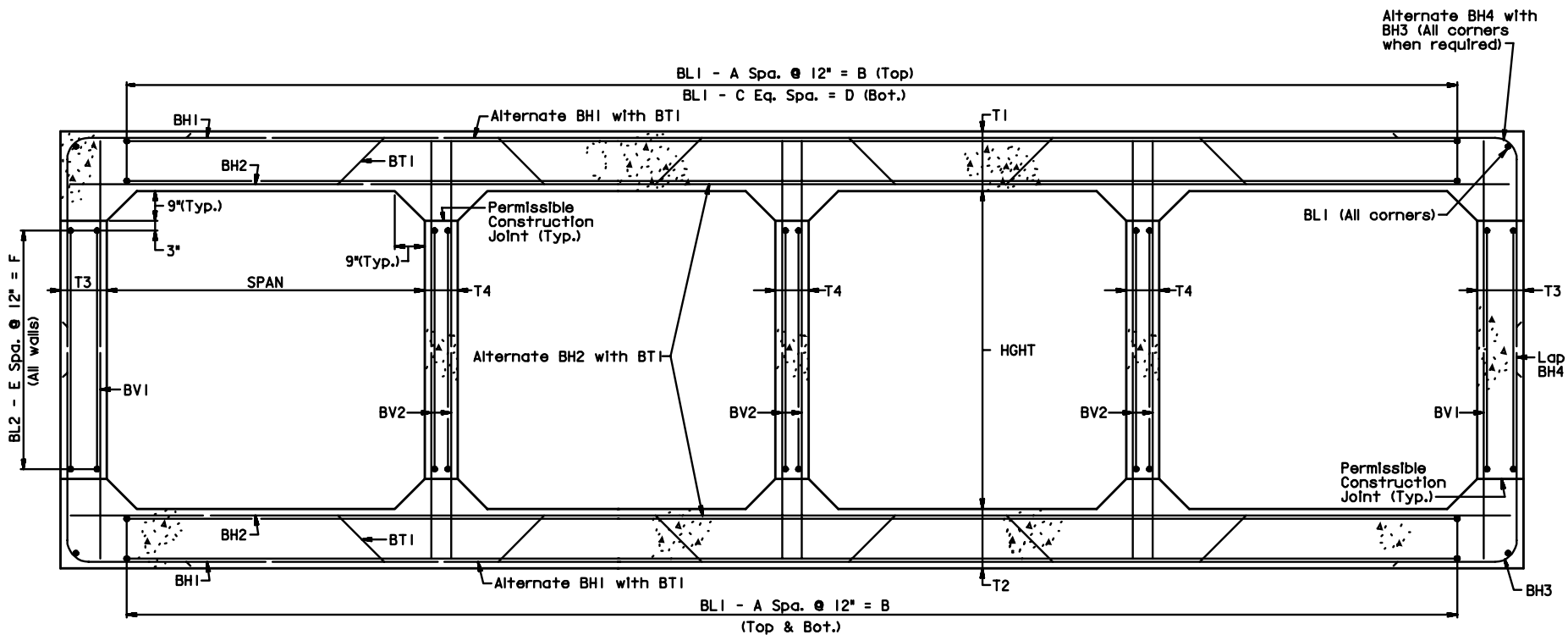
TYPICAL SECTION
