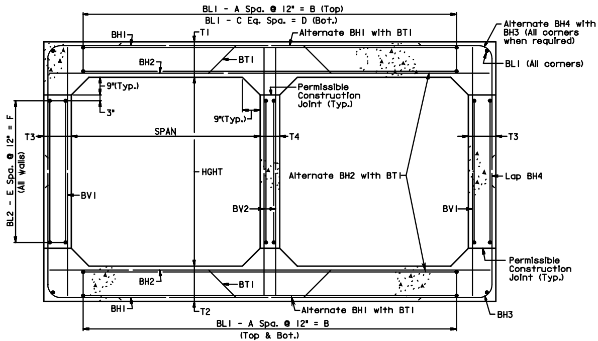
TYPICAL SECTION
