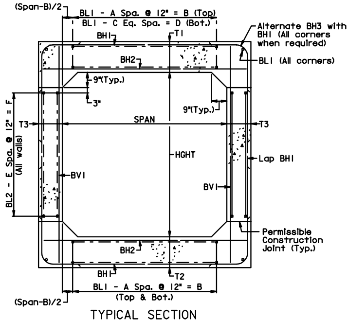
TYPICAL SECTION
