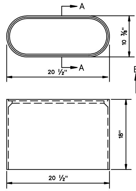
WATER METER BOX FOR 5/8" THRU 1" METER
