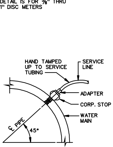
C.I./D.I. TAP INSTALLATION
