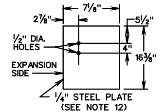
ANCHOR SLAB TYPE II END PLATE DETAIL
