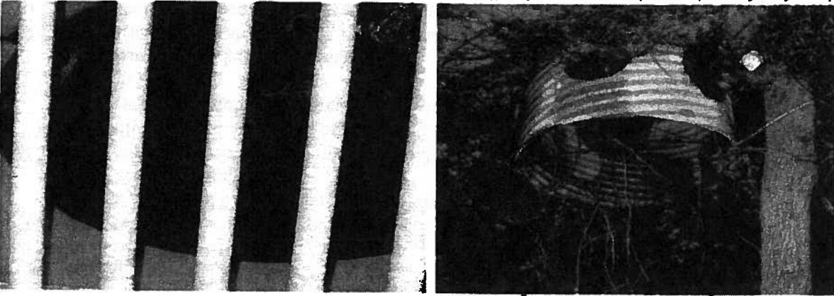
Riser chamber w/excessive amount of sediment Riser chamber clear of sediment & trash
