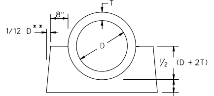
CONCRETE CRADLE
