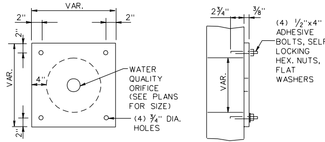
METAL PLATE DETAIL (NOT GALVANIZED)
