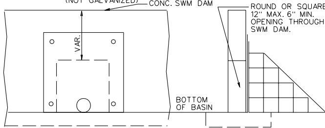
DETAIL FOR METAL PLATE AND WATER QUALITY ORIFICE TYPICAL SWM DAM SIDE VIEW OF SWM DAM WITH DEBRIS
