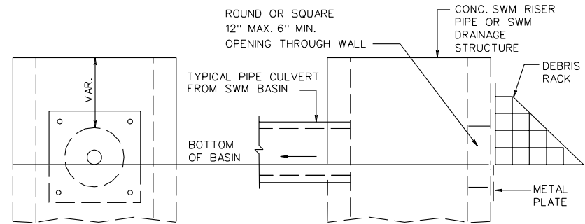
DETAIL FOR METAL PLATE AND WATER QUALITY ORIFICE SIDE VIEW WITH DEBRIS RACK TYPICAL SWM DRAINAGE STRUCTURE
