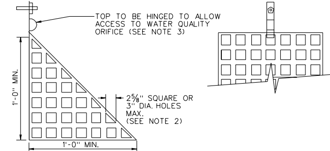
DETAIL FOR DEBRIS RACK (FOR WATER QUALITY ORIFICE)
