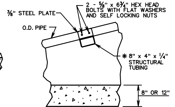
CENTER SUPPORT
