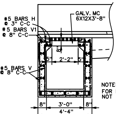
SECTION C-C
