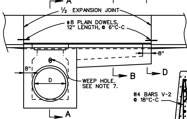
FRONT ELEVATION (PAVEMENT REMOVED)
