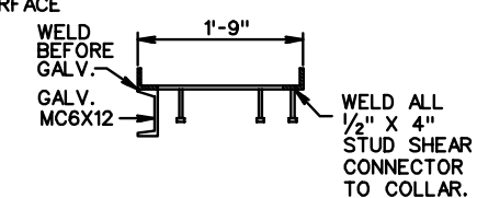
SECTION E-E
