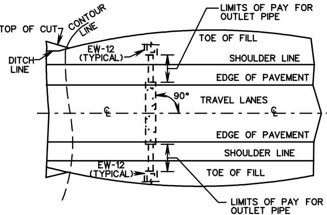
PLAN VIEW SHOWING PLACEMENT OF CD-2 UNDERDRAIN
