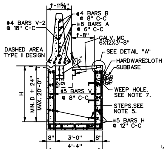
SECTION A-A (PIPE NOT SHOWN)
