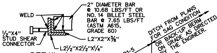
DETAIL A
