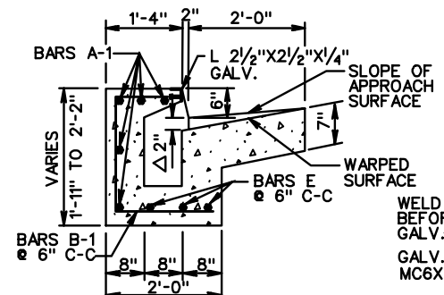
SECTION C-C
