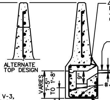
SECTION A-A (PIPE NOT SHOWN)
