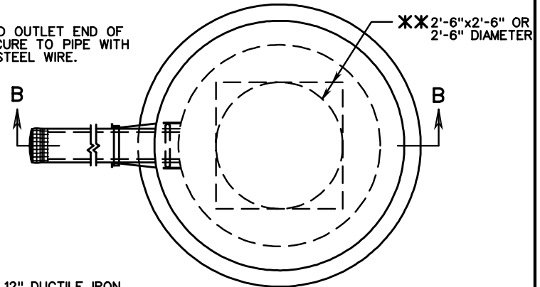
PLAN (CIRCULAR)
