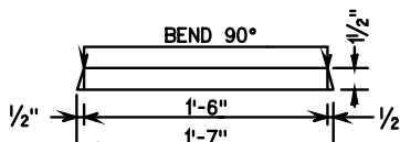
DETAIL D
