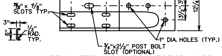
W-BEAM TERMINAL CONNECTOR (MOD.)
