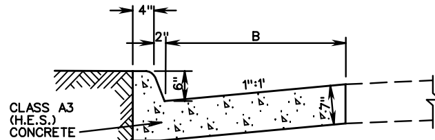
SECTION C-C
