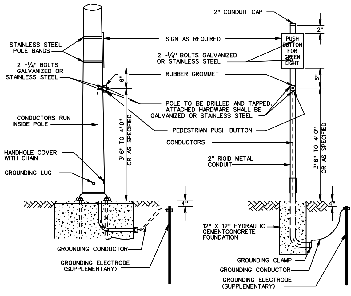
PA-2 SIGNAL/PEDESTAL POLE
