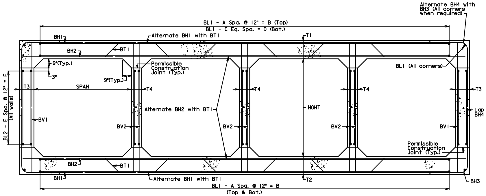
TYPICAL SECTION
