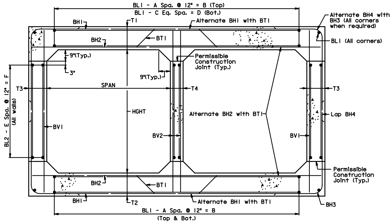
TYPICAL SECTION
