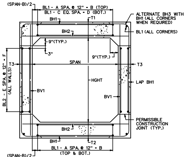
TYPICAL SECTION
