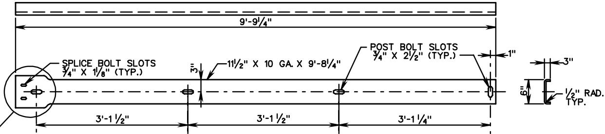
ITEM ⑦ DETAIL
