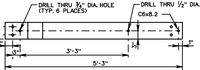
ITEM ⑧ DETAIL
