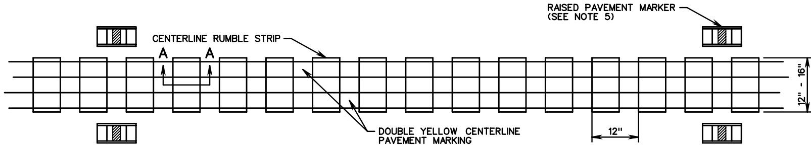
PLAN VIEW
