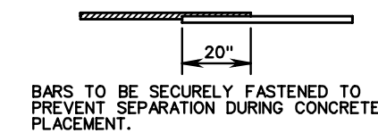
TYPICAL LONGITUDINAL LAP
