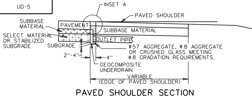
PAVED SHOULDER SECTION
