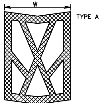
SEALANTS FOR TRANSVERSE CONTRACTION JOINTS
