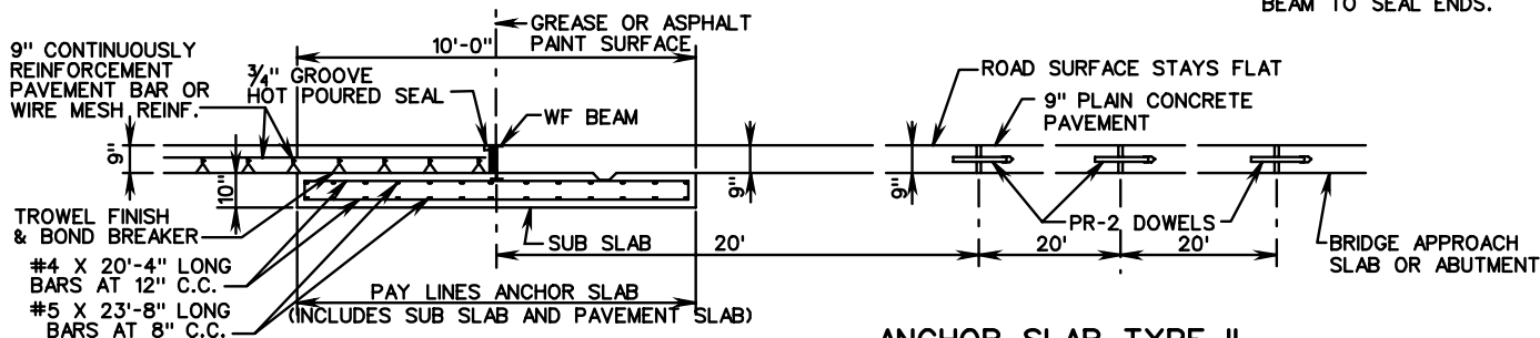
SECTION A-A ANCHOR SLAB TYPE II (FOR USE ADJACENT TO PLAIN CONCRETE PAVEMENT)
