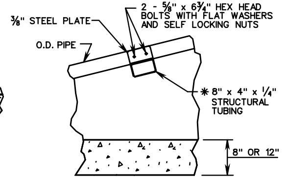
CENTER SUPPORT
