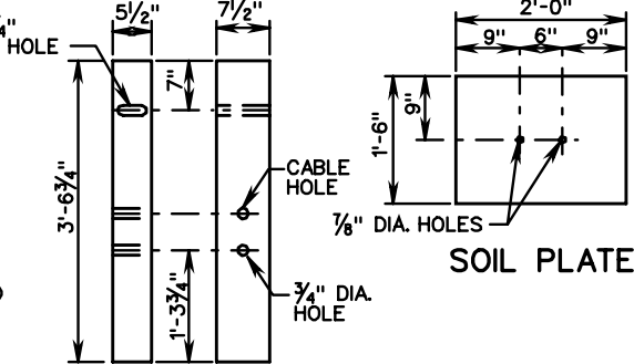
SHORT WOODEN POST
