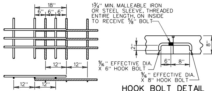
HOOK BOLT DETAIL
