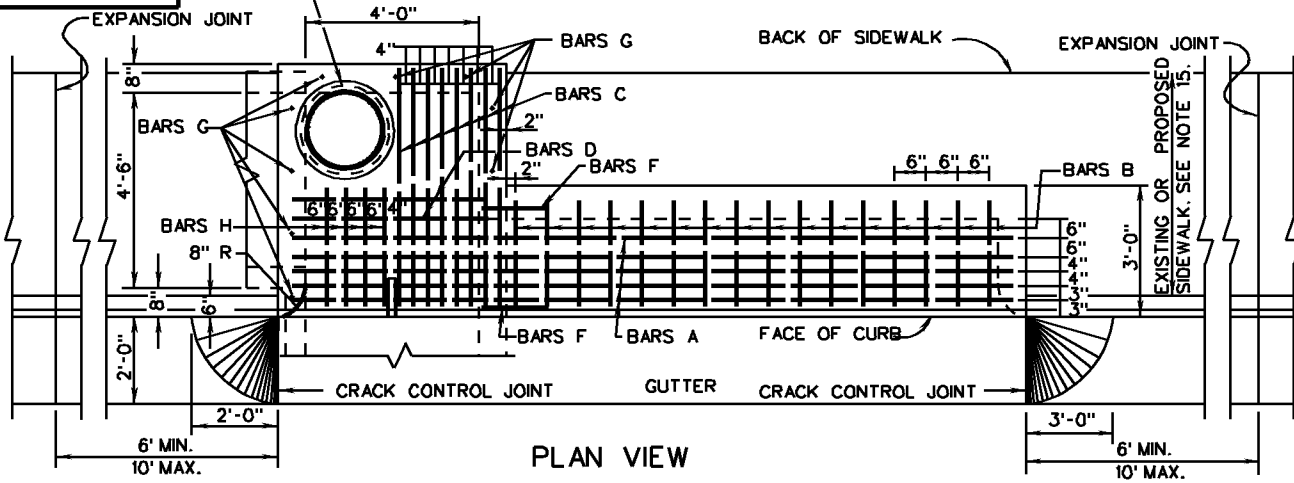
NOSE DETAILS
