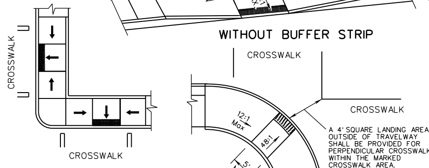
TYPICAL PLACEMENT AT INTERSECTION WITHIN CROSSWALK
