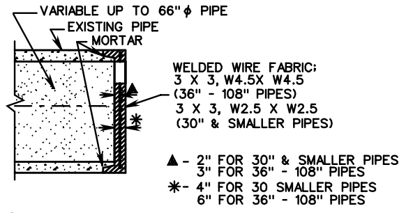
SECTION OF PRECAST PIPE PLUG (Male End) (MALE OR FEMALE PLUG DESIGN) TO BE FURNISHED WHERE APPLICABLE.
