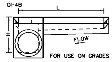
FRONT ELEVATION VIEW (GUTTER REMOVED)
