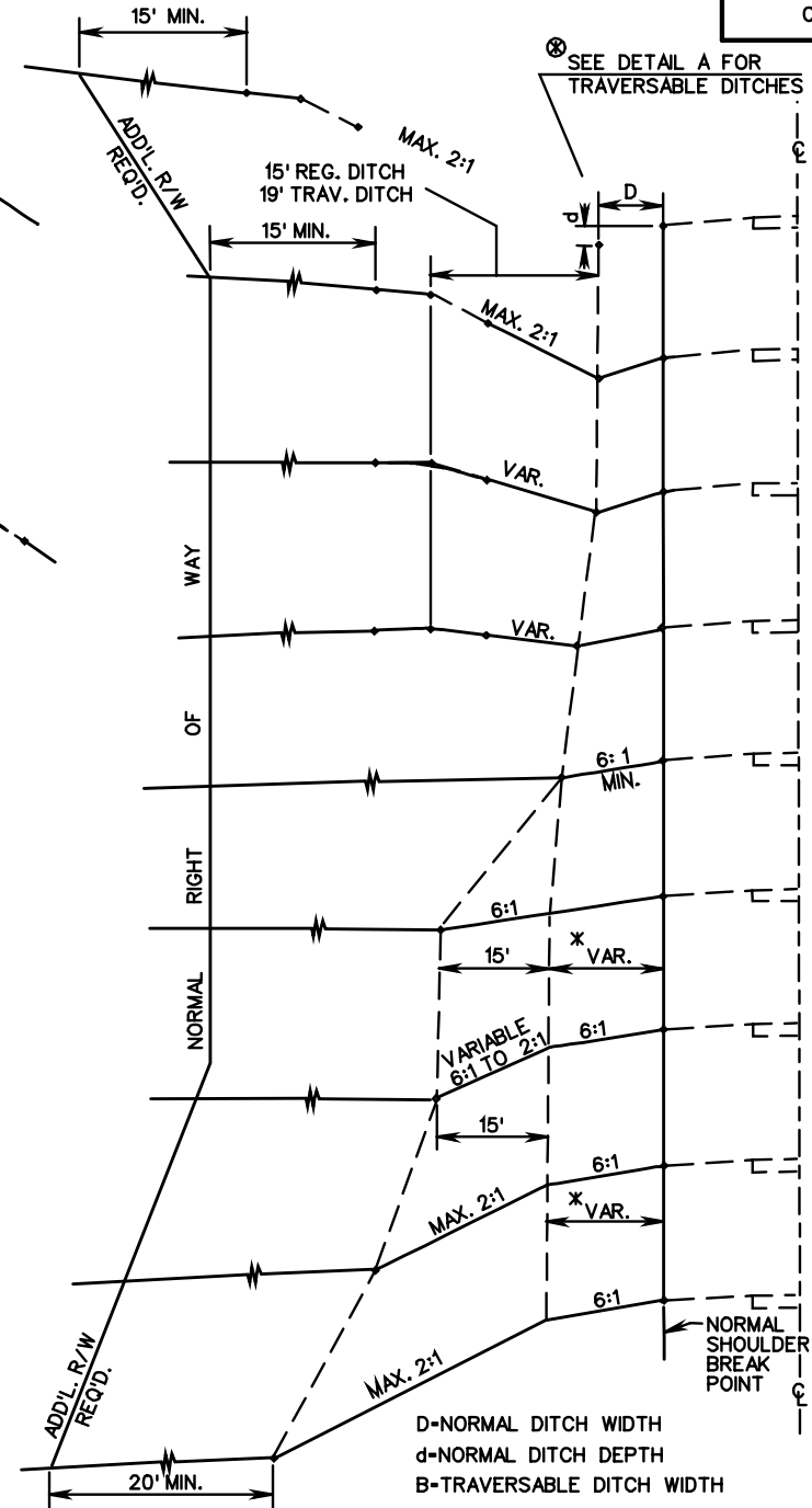
DETAIL SHOWING BERM DITCH IF SHOWN ON PLANS OR REQ'D. BY THE ENGINEER
