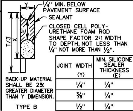
SEALANTS FOR TRANSVERSE CONTRACTION JOINTS
