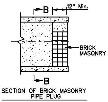
SECTION OF BRICK MASONRY PIPE PLUG
