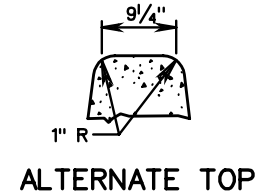
ISOMETRIC VIEW
