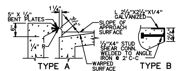
NOSE DETAILS
