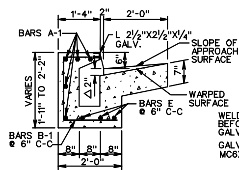
SECTION C-C Δ DECREASE TO 1" WHEN INLET IS USED WITH MEDIANS.
