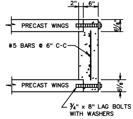
END WALL DETAIL
