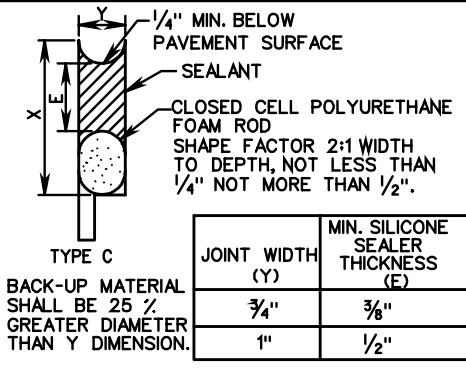
SEALANTS FOR TRANSVERSE EXPANSION JOINTS
