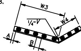
GRATE (GALVANIZED)
