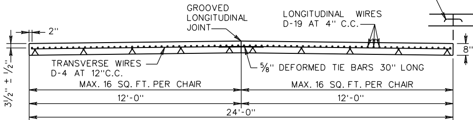
TRANSVERSE SECTION
