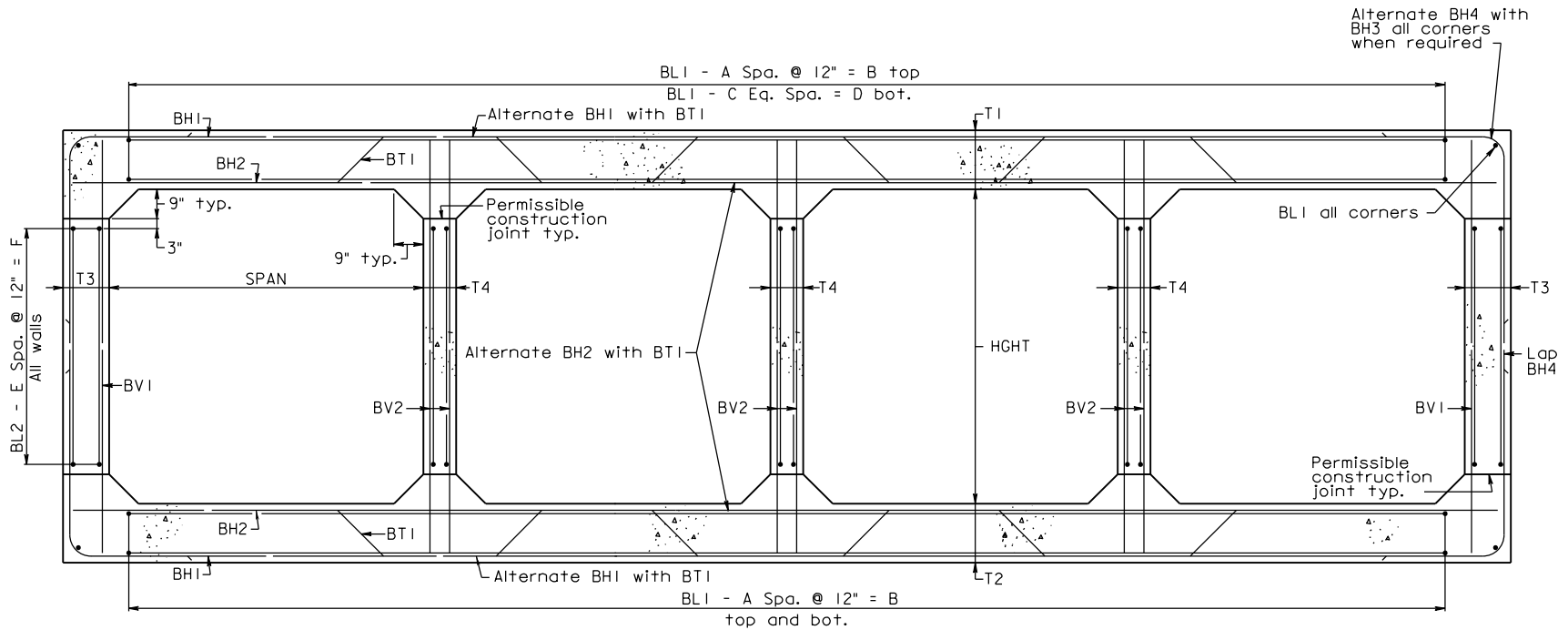
TYPICAL SECTION
