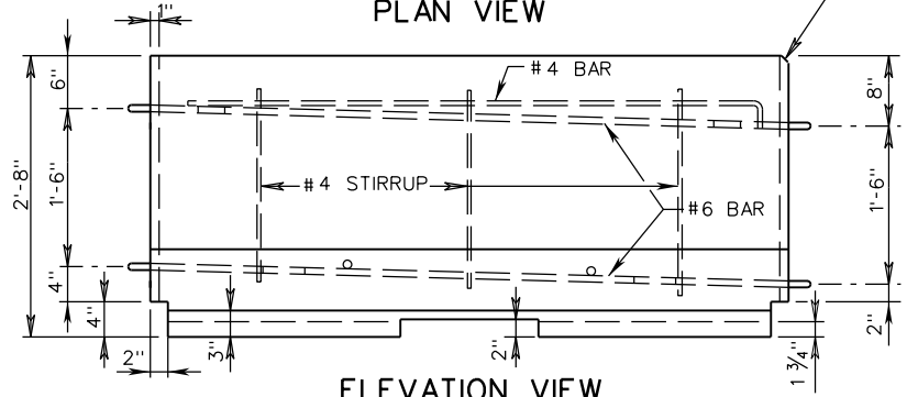
ELEVATION VIEW
